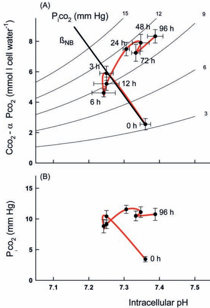
Figure 9.1 pH bicarbonate diagram (A) depicting the interrelated changes of intracellular acid-base variables pH ( pH_i ), bicarbonate and P_{CO_2} ( P_{iCO_2} ) over time and in relation to the non-bicarbonate buffer ( \beta_{NB} ) line. Initial changes in pH_i are driven by the accumulation of CO 2 which leads to a rise in P_{CO_2} (B), titrates non-bicarbonate buffers and is therefore paralleled by an accumulation of bicarbonate (A). Transmembrane ion exchange and metabolic processes interfere after 3 h and, after an initial base loss, lead to continued net bicarbonate accumulation while the respiratory acidosis persists with more or less constant P_{iCO_2} levels (based on data from Pörtner et al. , 1998).
