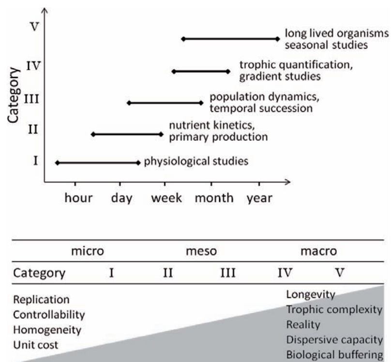
Figure 6.4 Size categories of ecosystem enclosures and duration of experiments in relation to relevant biological processes (SCOR Working Group 85, 2 nd Report, 1991).
