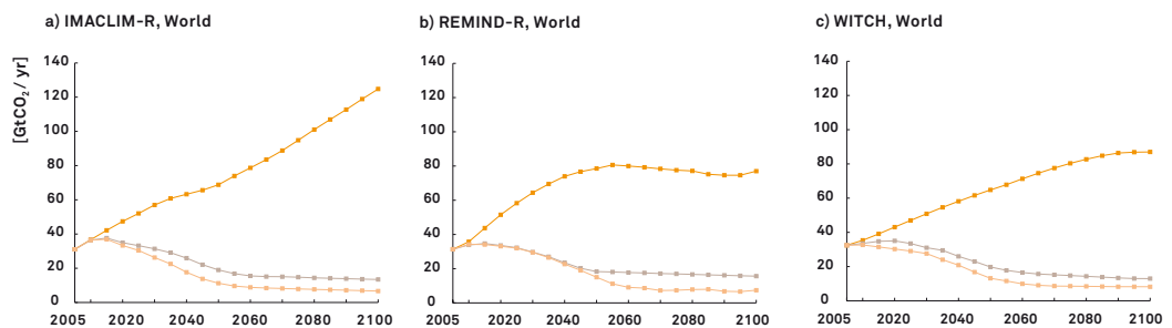
FIGURE 2-2 Global pathways for CO 2 emissions from fossil fuel combustion for the baseline scenario as well as policy scenarios aiming at stabilization of atmospheric CO 2 concentrations at 450 ppm and 410 ppm only calculated by IMACLIM-R, REMIND-R and WITCH
