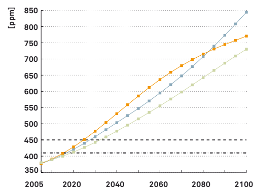
BASELINE, WORLD, CO 2 -CONCENTRATION
