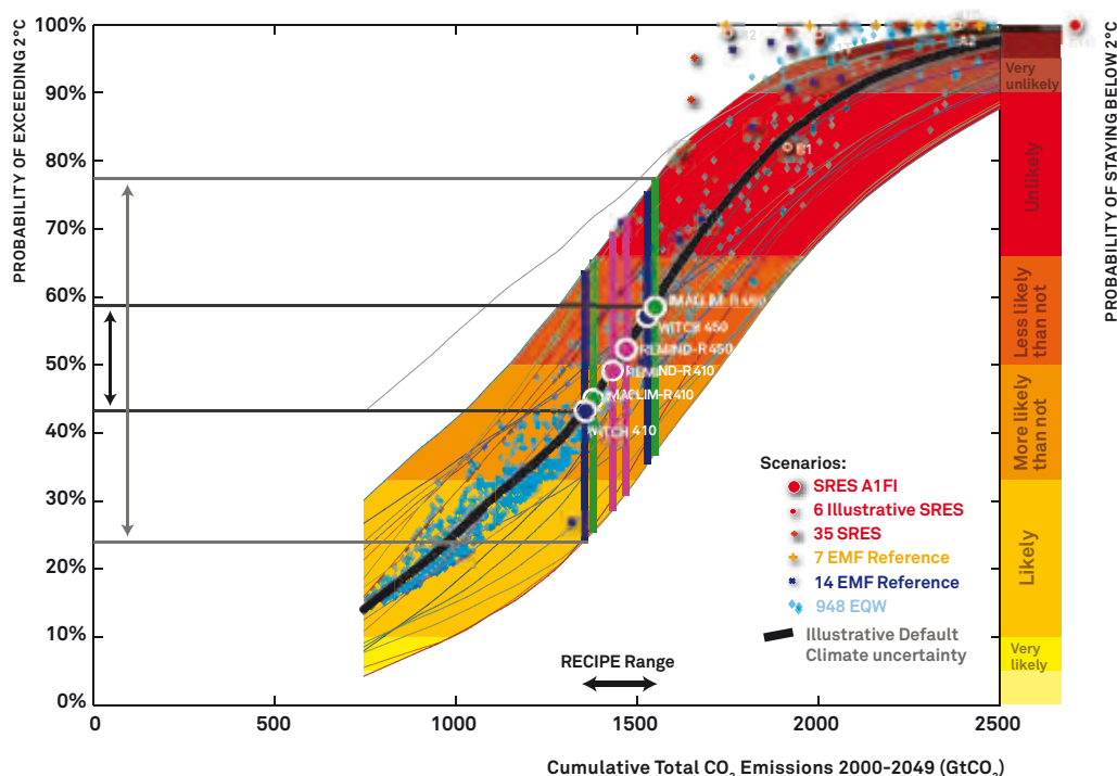
b) Probability of exceeding 2°C warming versus CO 2 emitted in the first half of the 21 st century as calculated by Meinshausen et al. (2009). According to this metric, RECIPE emission budgets until 2050 yield a medium likelihood of limiting warming to less the 2°C
