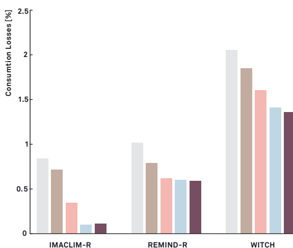
FIGURE 2-9 Global mitigation costs (displayed as consumption losses) for various scenarios with delayed participation in a global carbon market, and a benchmark case with global participation from 2010. Percentage changes are relative to baseline using a 3% discount rate
