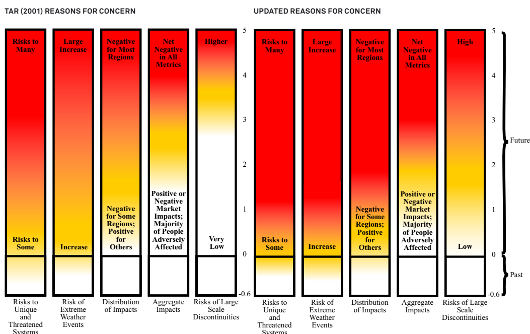
FIGURE 1-1 Risks from climate change by reason for concern, as appraised by the IPCC Third Assessment report compared with recently updated data. Climate change impacts are depicted against increases in global mean temperature (°C) after 1990 (Smith et al., 2009)
