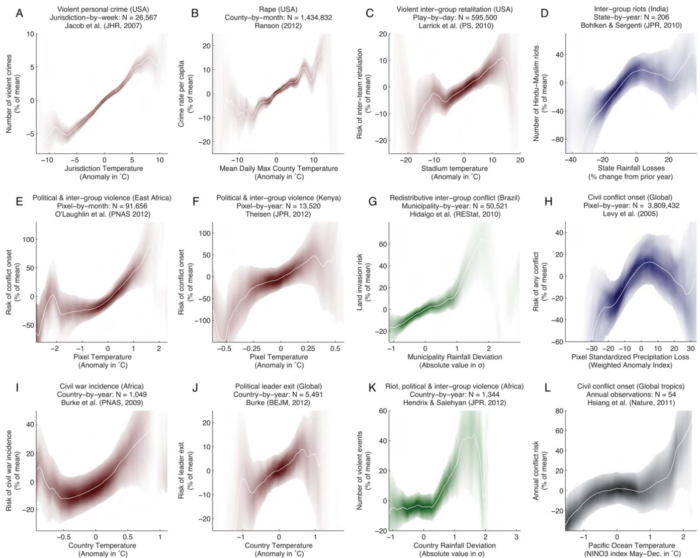
Fig. 2. Empirical studies indicate that climatological variables have a large effect on the risk of violence or instability in the modern world. Examples from studies of modern data that identify the causal effect of climate variables on human conflict. Both dependent and independent variables have had location-effects and trends removed, so all samples have a mean of zero. Relationships between climate and conflict outcomes are shown with non-parametric “watercolor regressions”, where the color intensity of 95% confidence intervals depicts the likelihood that the true regression line passes through a given value (darker is more likely) (128). White line is the conditional mean (129, 130). Climate variables are indicated by color: red = temperature, green = rainfall deviations from normal, blue = precipitation loss, black = ENSO. Panel titles describe the outcome variable, location, unit of analysis, sample size and study. Because the samples examined in each study differ, the units and scales change across each panel (see Figs. 4 and 5 for standardized effect-sizes). “Rainfall deviation” represents the absolute value of location-specific rainfall anomalies, with both abnormally high and abnormally low rainfall events described as having a large rainfall deviation. “Precipitation Loss” is an index describing how much lower precipitation is relative to the prior year or long-term mean.
