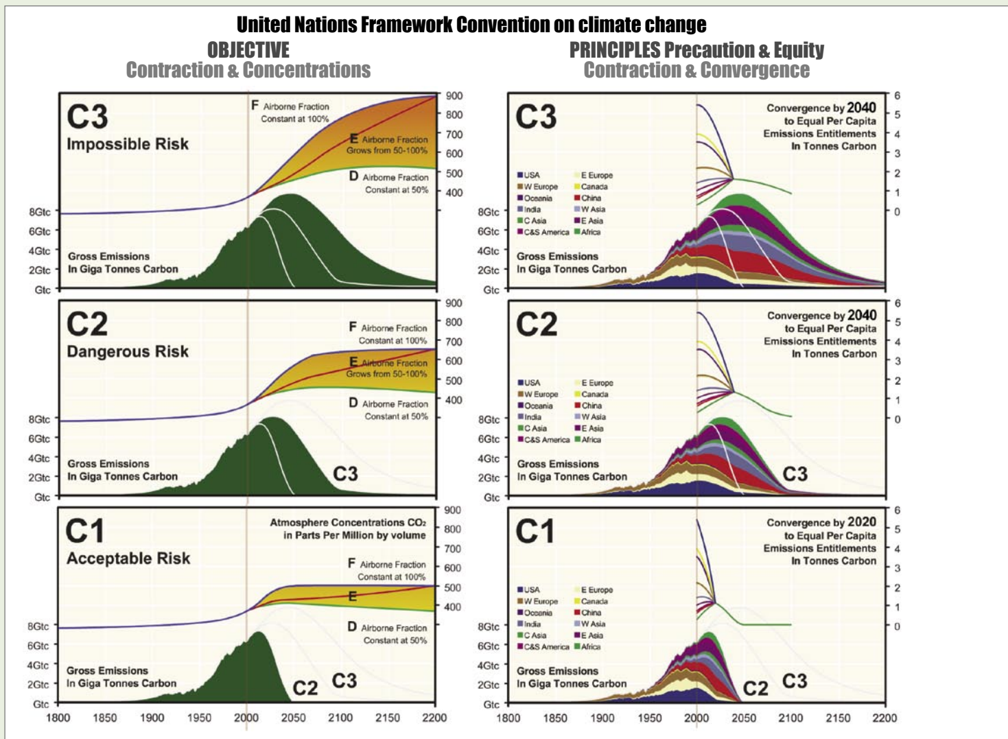
Figure 2: Charting the UNFCCC Objective & Principles, the Development Benefits of Growth versus the growth of Climate Change Related Damage Costs. ( http://www.gci.org.uk/images/Proportionate_Response.pdf )
